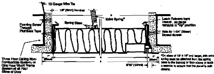
FIGURE 2 3-HOUR CEILING INSTALLATION DETAIL MODELS FD, FDSS, REFER TO TABLE
